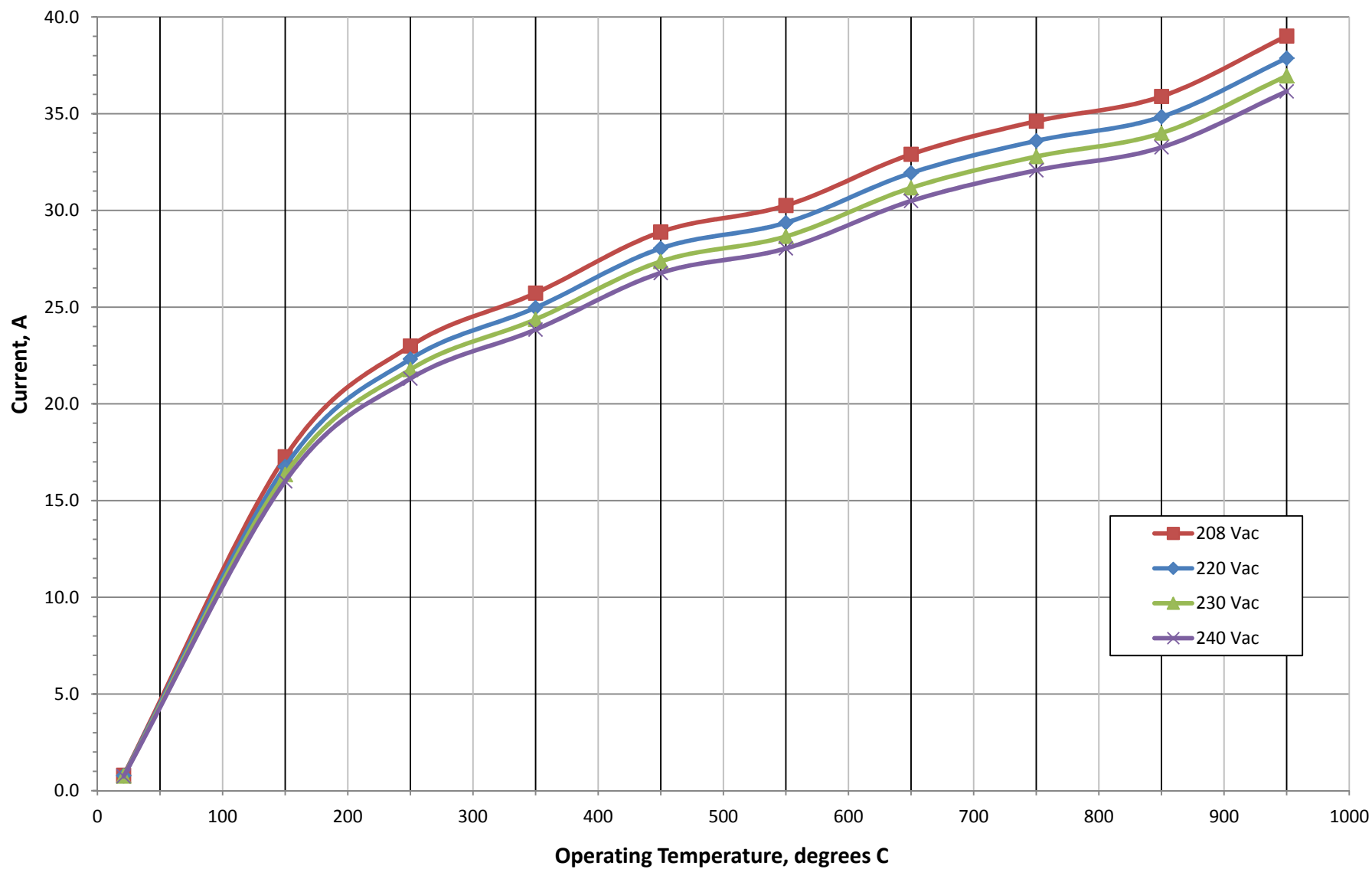
LA-306 Average 1-PH Current at Operating Temperatures
