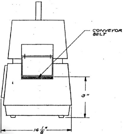
ENTRANCE ELEV
